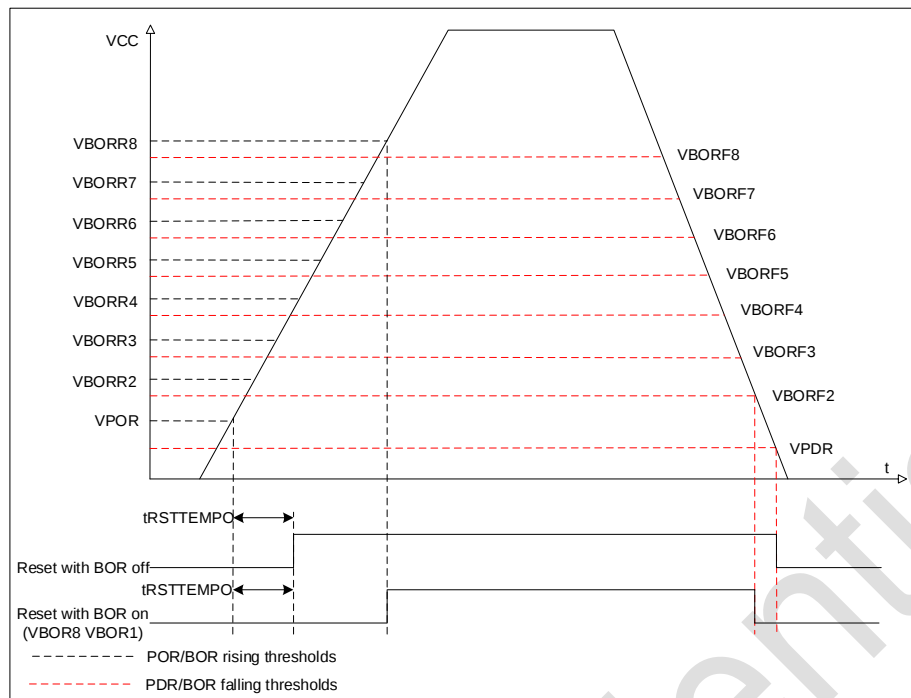
Figure 2-3 POR/PDR/BOR threshold
