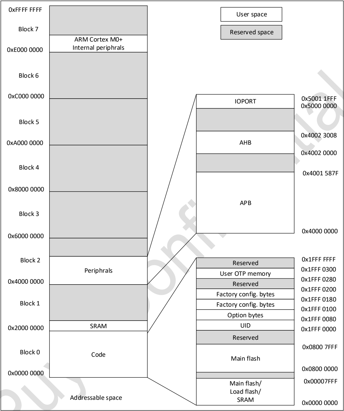
Figure 4-1 Memory map
